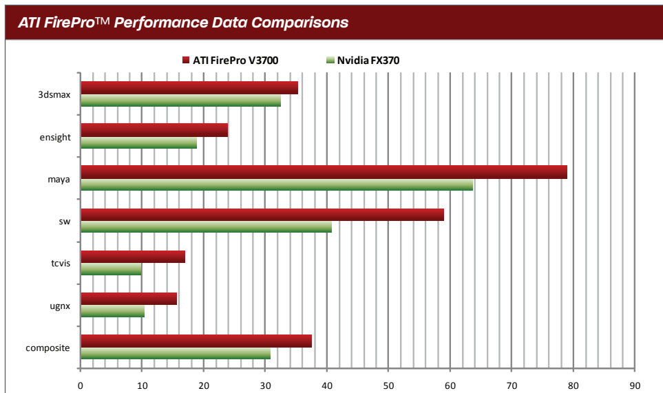
Average of all eight SPECviewPerf 10 tests using Nvidia published scores. http://nvidia.com/object/fo_11761.html
